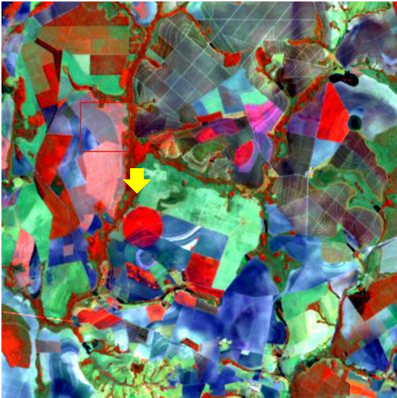
Landsat-5/TM-09
